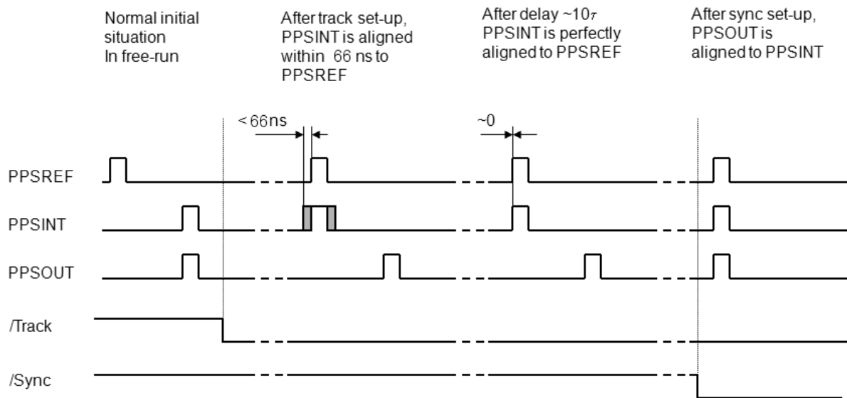
Figure 2.4-2 “Track” mode and “Sync” mode.
