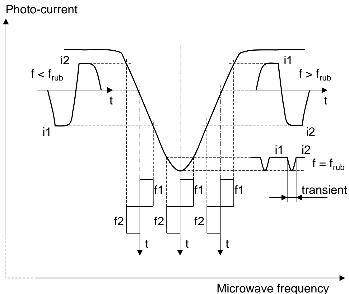
Figure 2.3-1 Dip minimum detection.
