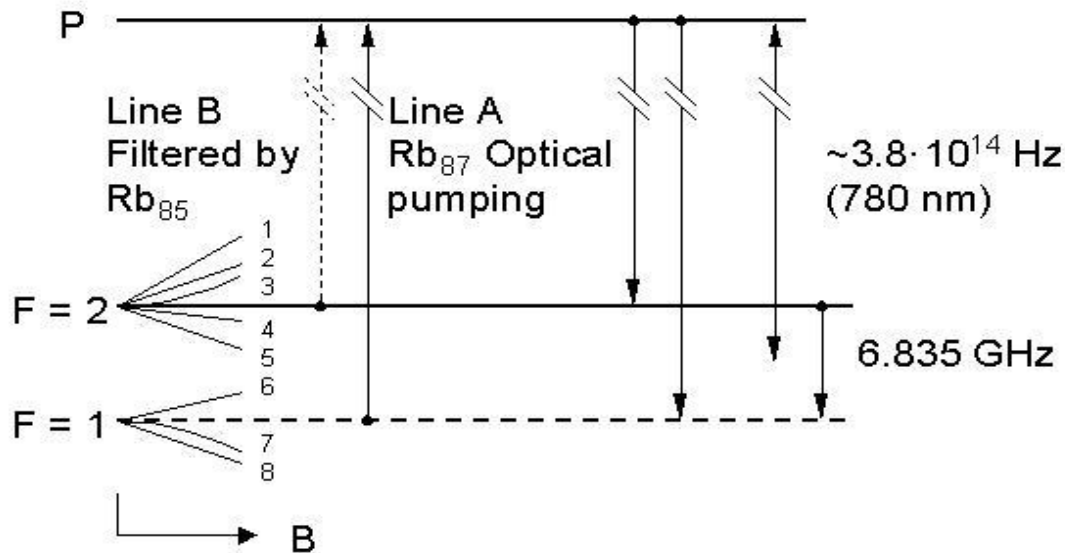
Figure 2.1-1 Energy levels and transitions in Rb87 atoms during LNRCLOCK operation.
