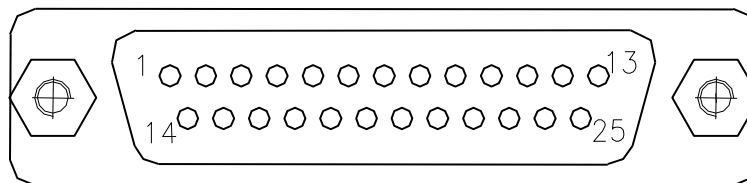
Figure 4.4-1 J2 Sub-D pin connector of LNRClOk-100.
