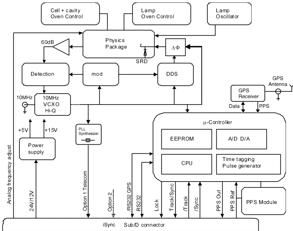
Figure 2.3-2 LNRClOk bloc diagram.
