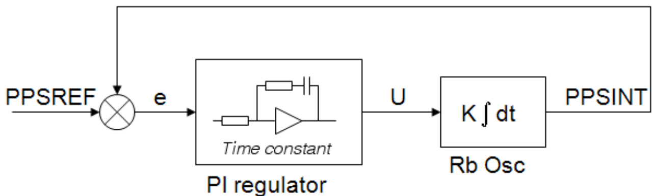
Figure 2.4-3 Schematic of the PPSREF regulation loop.
