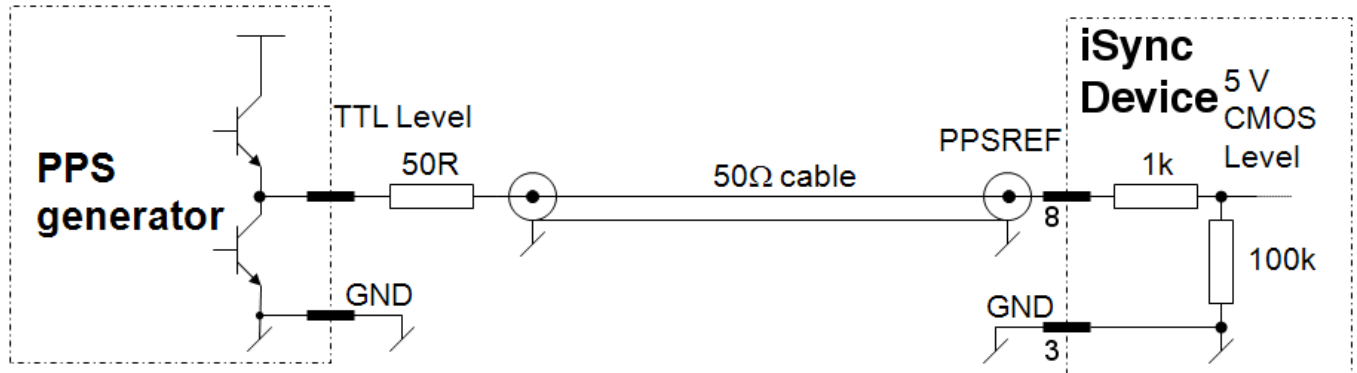
Figure 4.20-1 This schematic is recommended to connect a PPSREF to the LNRCLCLOCK on distances up to 10m.
